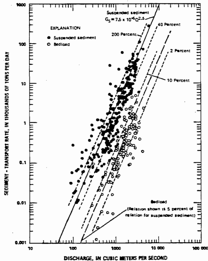
Fig. 3 Sediment transport rate as a function of discharge, Snake and Clearwater rivers in the vicinity of Lewiston, Idaho.
