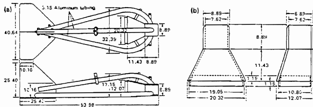
Fig. 2 Plan and side elevation drawings of (a) 7.62 cm Helley-Smith bed load sampler, and (b) sampler nozzle. All dimensions in centimetres.
