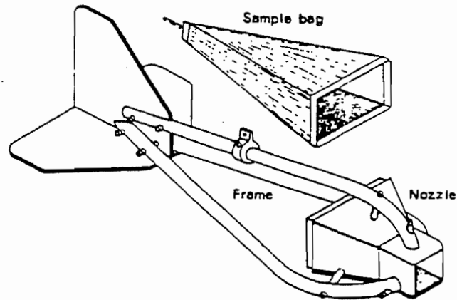
Fig. 1 Helley-Smith bed load sampler.
