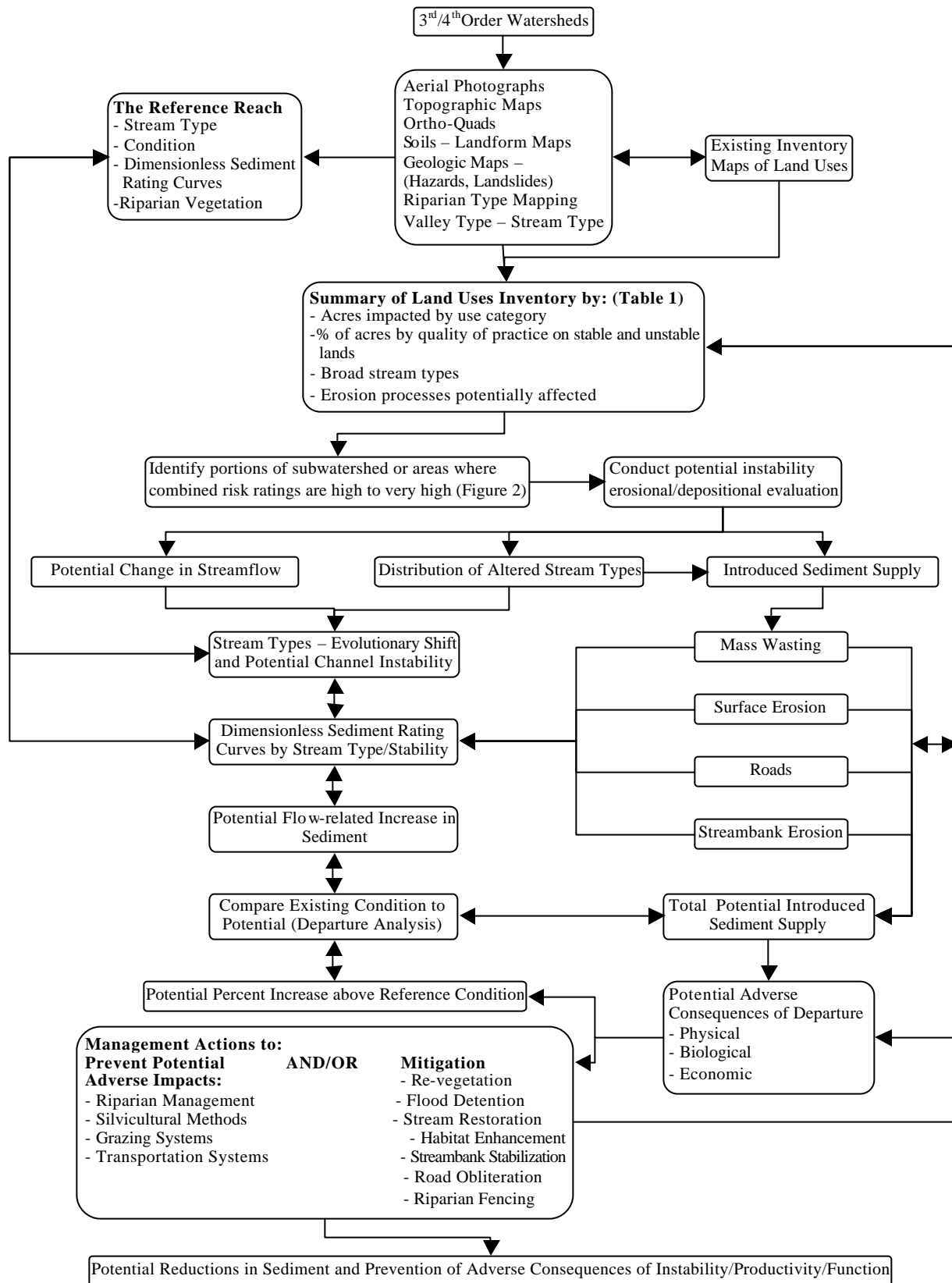
Figure 1. The Broad and/or Initial Level of Assessment
