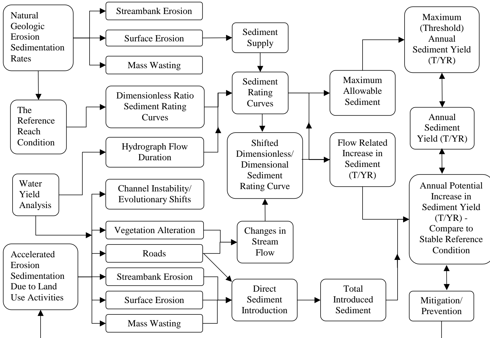
Figure 3. The Intermediate Level of Assessment Showing Prediction Comparison of Natural Geologic Rates of Sediment Compared to Potential Increases due to Land Use Activities (from: Rosgen, 1999).
